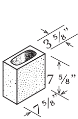
HALF 4" x 8" x 8"
