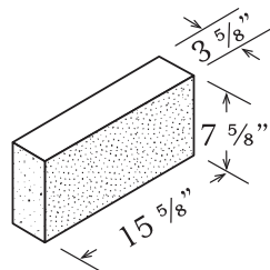
SOLID 4" x 8" x 16"
