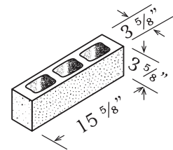
HALF HEIGHT STRETCHER 4" x 4" x 16"
