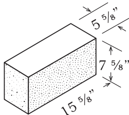
SOLID 6" x 8" x 16"
