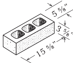
HALF HEIGHT 6" x 4" x 16"
