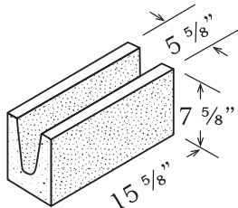
BOND BEAM 6" x 8" x 16"
