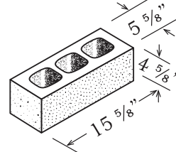
STARTER 6" x 5" x 16"
