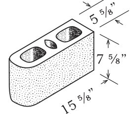
DOUBLE END BULLNOSE 6" x 8" x 16" - Splittable
