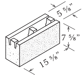
KNOCK-OUT 6" x 8" x 16"
