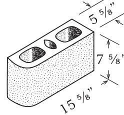
SINGLE BULLNOSE 6" x 8" x 16" - Splittable
