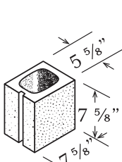
HALF 6" x 8" x 8"
