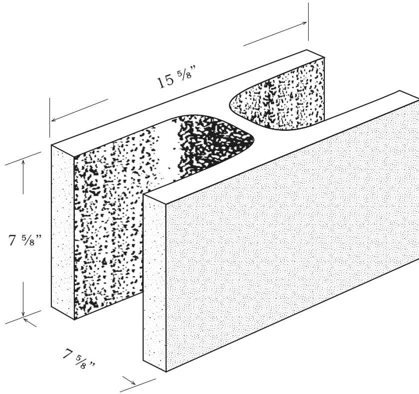
HALF SASH 8" x 8" x 16"
