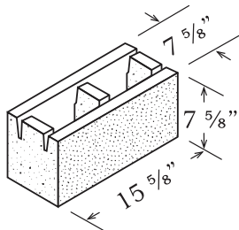
KNOCK OUT BOND BEAM 8" x 8" x 16"
