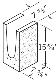
LINTEL 8" x 16" x 8"
