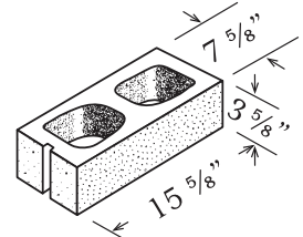
HALF HEIGHT 2 CORE 8" x 4" x 16"
