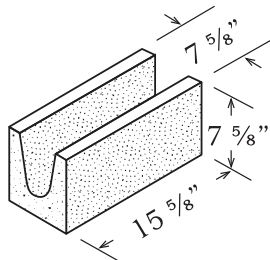
BOND BEAM 8" x 8" x 16"
