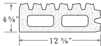
CORNER BLOCK
