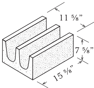
DOUBLE BOND BEAM 12" x 8" x 16"
