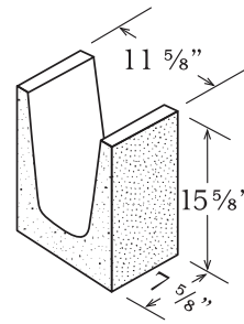
LINTEL 12" x 16" x 8"
