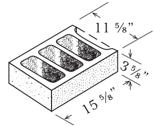
HALF HEIGHT STRETCHER 12" x 4" x 16"
