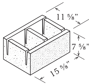
KNOCK OUT BOND BEAM 12" x 8" x 16"
