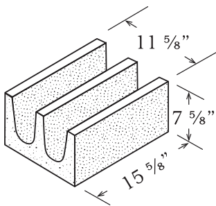
DOUBLE BOND BEAM 12" x 8" x 16"
