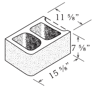
SINGLE BULLNOSE 12" x 8" x 16"
