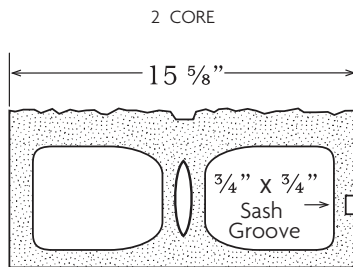
8" x 8" x 16" Splittable
