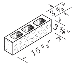
HALF HEIGHT STRETCHER 4" x 4" x 16"
