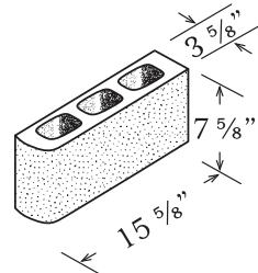
SINGLE BULLNOSE 4" x 8" x 16"
