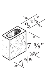
HALF 4" x 8" x 8"
