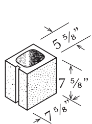
HALF 6" x 8" x 8"
