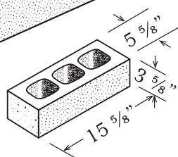
HALF HEIGHT 6" x 4" x 16"
