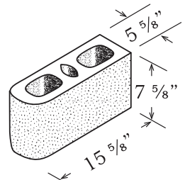
DOUBLE END BULLNOSE 6" x 8" x 16" - Splittable
