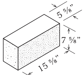
SOLID 6" x 8" x 16"
