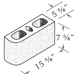
SINGLE BULLNOSE 6" x 8" x 16" - Splittable
