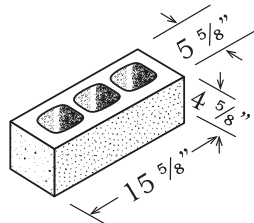
STARTER 6" x 5" x 16"
