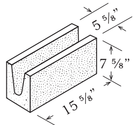
BOND BEAM 6" x 8" x 16"
