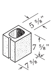
HALF 6" x 8" x 8"
