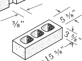
HALF HEIGHT 6" x 4" x 16"
