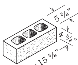
STARTER 6" x 5" x 16"
