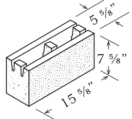
KNOCK-OUT 6" x 8" x 16"
