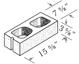
HALF HEIGHT 2 CORE 8" x 4" x 16"
