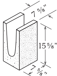
LINTEL 8" x 16" x 8"
