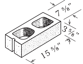
HALF HEIGHT 2 CORE 8" x 4" x 16"
