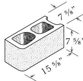
SINGLE BULLNOSE 8" x 8" x 16"
