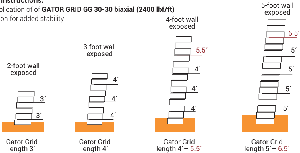
4" block built with 3:1 slope in clay soil condition
