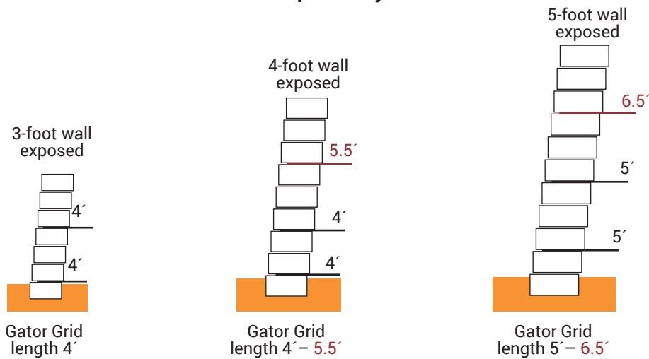
6" block built with 3:1 slope in clay soil condition
