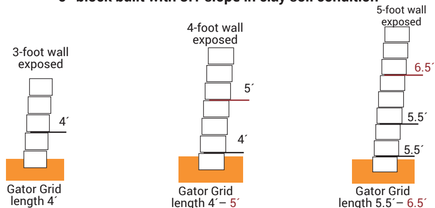
8" block built with 3:1 slope in clay soil condition
