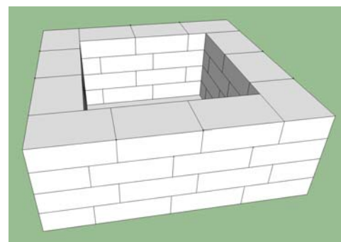
4th Course 12 block
